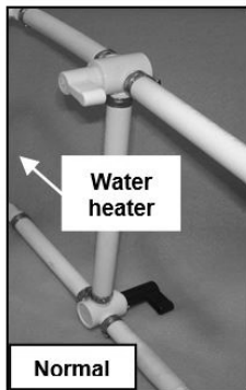
Two Valve Water Heater Bypass
