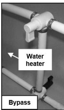
Two Valve Water Heater Bypass
